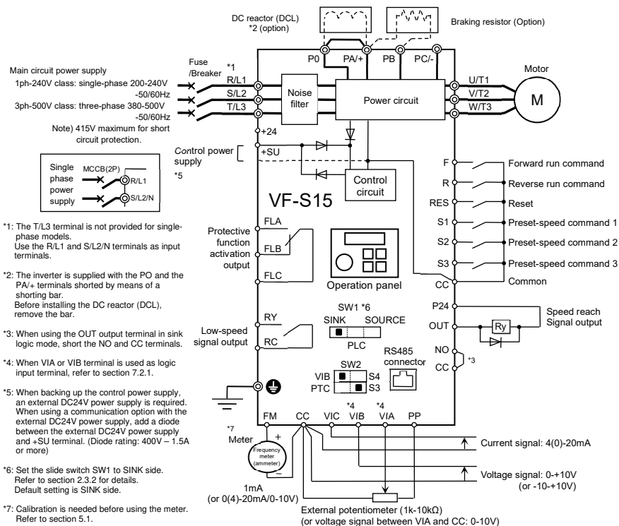
Standard connection diagram – SINK with internal supply (Negative) (common: CC)
